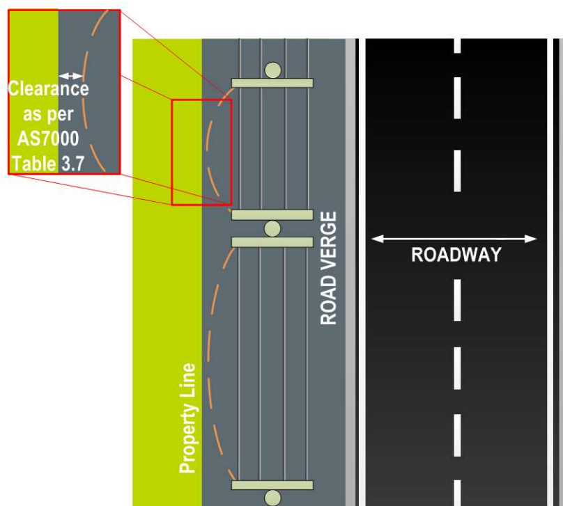
Figure 5 - Roadway requirements
